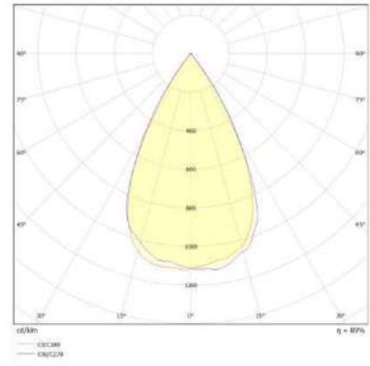
60 Derece Lens / 60 Degree Lens
